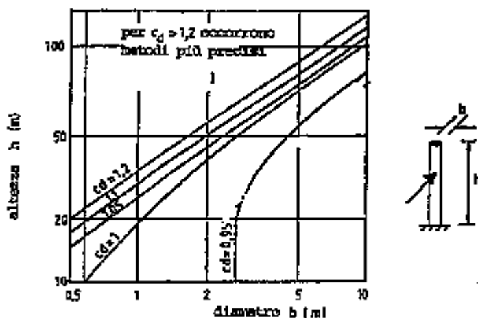
Fig C.7.11. (c) - Ciminiere in c.a.
